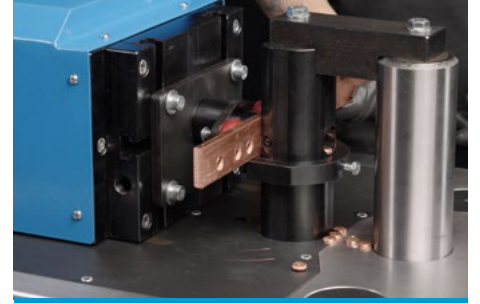
BARA DELME APARATI BUSBAR PUNCHING TOOL
